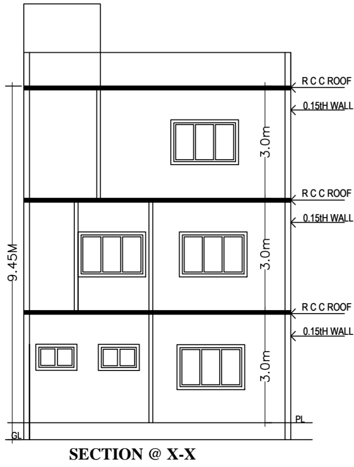
SECTION @ X-X
